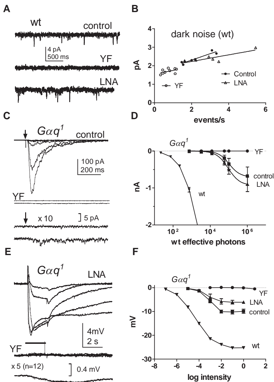
Figure 7. Suppression of dark noise and responses in Gaq mutants by YF diet. A , Whole-cell patch-clamped recordings from wild-type photoreceptors in the dark. When reared on normal diet (control) or LNA diet, spontaneous \sim 2 pA events occurred at \sim 2 –4 events s^{-1} . These were greatly suppressed on YF diet. B , Scatter plot of event rate and amplitude from flies reared on YF ( n = 9 cells), control ( n = 6 cells), and LNA diets ( n = 5 ). C , Photoreceptor whole-cell recordings from Gaq 1 hypomorphs. Top traces, Responses from flies reared on control diet, to 10 ms flashes (arrows) increasing in intensity from \sim 750 to 10^6 effective photons (wild-type calibration). Middle, Responses from two representative Gaq 1 cells reared on YF diet to flashes of brightest intensity ( \sim 10^6 photons) on the same scale and shown again below on 10\times higher gain. One cell had no response, the other a slow \sim 4 pA response. D , Response intensity function (peak currents) from Gaq 1 flies reared on control diet (mean \pm SEM; n = 5 cells), YF diet ( n = 12 ), and LNA diet ( n = 9 ). Data also shown for wild-type photoreceptors (LNA diet, n = 4 ), which are \sim 1000\times more sensitive. E , ERG recordings from Gaq 1 hypomorphs in response to 2 s flashes (bar) of increasing intensity. Top traces, Gaq 1 fly reared on LNA diet (log -4 to log 0). Middle traces, From a fly reared on YF diet (4 superimposed traces: log -3 to log 0). Bottom trace, Averaged response to 12 flashes of a higher intensity (log +1 ) at 5\times greater gain. F , Response intensity function of peak ERG responses from Gaq 1 reared on normal (control, n = 4 flies), YF ( n = 5 ), and LNA diets ( n = 4 flies) compared with wt fly reared on normal food.
