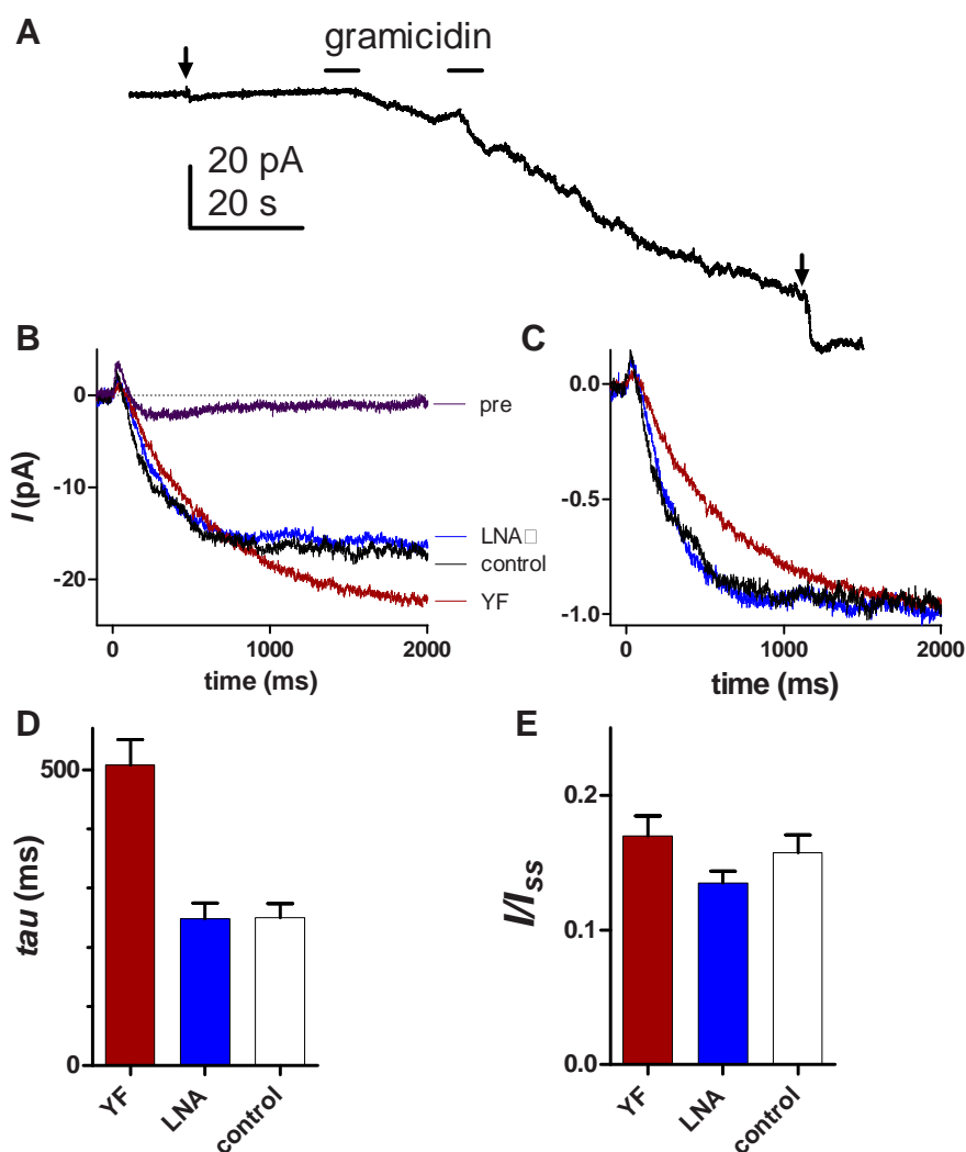
Figure 10. Responses mediated by mechanosensitive gramicidin channels. A , Representative whole-cell recording from a trpl mutant (reared on LNA diet) in bath containing \text{La}^{3+} (100 \mu\text{M} ) and ruthenium red (20 \mu\text{M} ) to ensure total blockade of the light-sensitive TRP channels. A 10 ms test flash ( \sim 10^5 effective photons, arrowhead) elicited a tiny residual biphasic current (see pre in B ). Two brief (4 s) applications of gramicidin (0.1 ng/ml) from a puffer pipette resulted in an inward current as gramicidin channels were incorporated into the membrane. After a constitutive (“steady-state”) current ( I_{ss} ) of \sim 70 pA had developed the same test flash now induced a rapid increase in the gramicidin-mediated current. B , Gramicidin-mediated responses (each averaged from 8 to 11 cells) to the 10 ms test flash (delivered at t = 0 ) in flies reared on normal diet (control), YF, and LNA diets; residual response ( n = 9 ) before gramicidin application (pre) shown for comparison. C , Same responses normalized to emphasize difference in kinetics. D , Time constants ( \tau ) of single exponentials fitted to the responses were \sim 2\times slower in flies raised on YF diet (mean \pm SEM; n = 9 –14 cells; p < 0.001 , one-way ANOVA, Bonferroni correction). E , Amplitudes of responses expressed as fraction of the steady-state gramicidin current ( I_{ss} ) were not significantly different.
