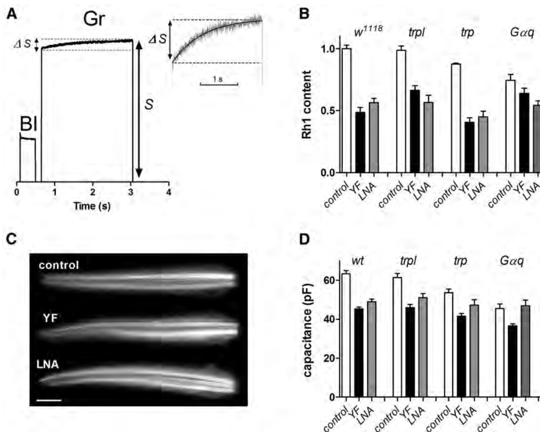
Figure 1. Diet has only minor effects on visual pigment and morphology. A , Reflectance/scattered light measurements from deep pseudopupil of intact white-eyed fly ( w 1118 ): rhodopsin was first converted to metarhodopsin (M) by bright blue (BI = 470 ± 20 nm) excitation, and then reconverted to the rhodopsin state (R) by long wavelength green illumination (Gr = 550 ± 50 nm). Because M absorbs maximally 570 nm and R at 480 nm, less long wavelength light is absorbed by the eye as M is photoreisomerized back to R and the intensity of the reflected/back-scattered green light (S) increases with an exponential time constant reflecting the rate of M → R conversion (inset on expanded scale). The relative increase during this phase ( \Delta S/S ) provides a measure of the concentration of visual pigment in the eye. B , Relative rhodopsin (Rh1) content in wild-type ( wt ), trpl , trp , and Gαq mutants derived from \Delta S/S values normalized to wild-type ( w 1118 ) control flies reared on normal diet. In most cases values for flies reared on both YF and LNA diets were reduced ~2-fold compared with control diet (white bars), but YF and LNA-reared flies in each genotype showed no significant differences from each other (one-way ANOVA). Mean ± SEM; n = 6–10 flies each. C , Dissociated ommatidia from flies reared on normal, YF, and LNA diets appeared similar (fluorescent micrographs of ommatidia from wild-type flies expressing GFP-tagged arrestin to highlight rhabdomeres). Scale bar, 10 μm. D , Whole-cell capacitances in wild-type, trpl , trp , and Gαq flies reared on control, YF, and LNA diets (mean ± SEM; n = 8–27 cells each). In each genotype, values on YF and LNA diets were statistically indistinguishable (one-way ANOVA), although usually slightly lower than on control diet.
