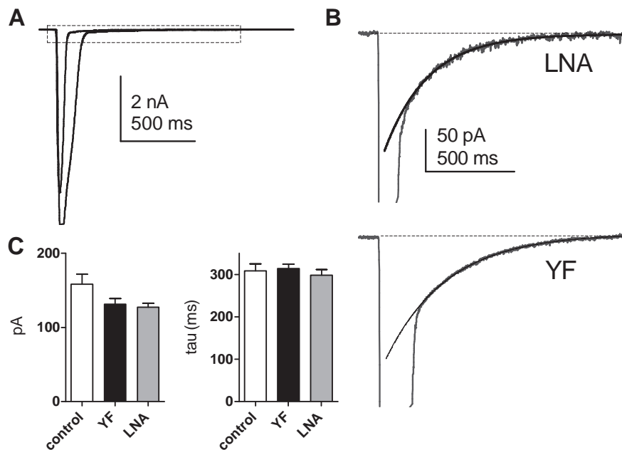
Figure 8. \text{Na}^+/\text{Ca}^{2+} exchanger currents are unaffected by diet. A , Whole-cell voltage-clamped responses to 10 ms flashes containing \sim 10^6 effective photons in wild-type photoreceptors reared on LNA and YF diet (broader response). B , Detail from same traces (boxed region) at higher gain reveals a slowly decaying aftercurrent due to electrogenic \text{Na}^+/\text{Ca}^{2+} exchanger activity extruding \text{Ca}^{2+} that entered during the light response (Chu et al., 2013a); currents fitted with a single exponential with time constant 261 ms (LNA) and 340 ms (YF). C , Summary of data: amplitude (pA) of the exchanger currents (extrapolated back to the peak of light response) and time constant of decay (tau) were similar across all diets. Mean \pm SEM, n = 10 (YF), 10 (LNA), and 5 cells (control diet). The larger currents on control diet are attributable to somewhat larger cells in this sample (mean capacitances: YF 45, LNA 47, and control 64 pF).
